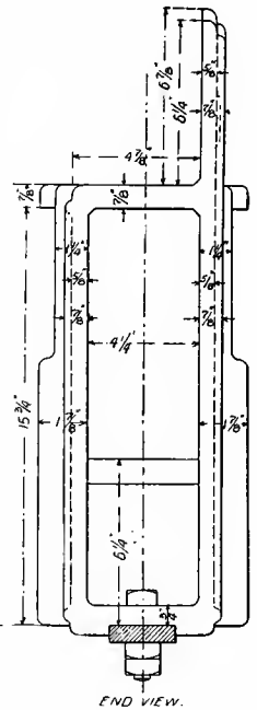
Fig. 5482. End Elevation.
